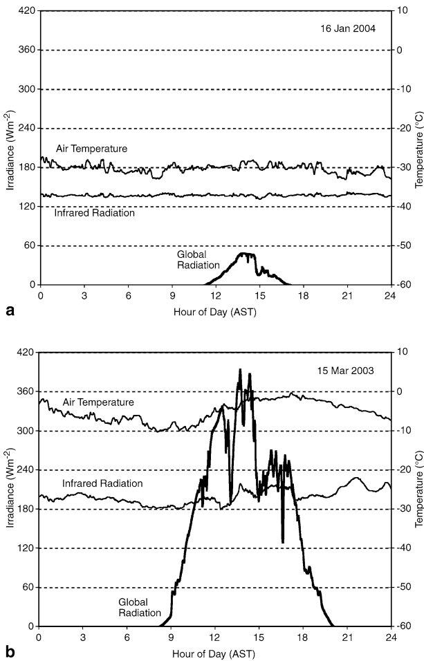
Fig. 8. Diurnal variation of the long wave incoming radiation and temperature on a winter (a) and spring (b) day with high-level cloud cover. Data in minute intervals are plotted
