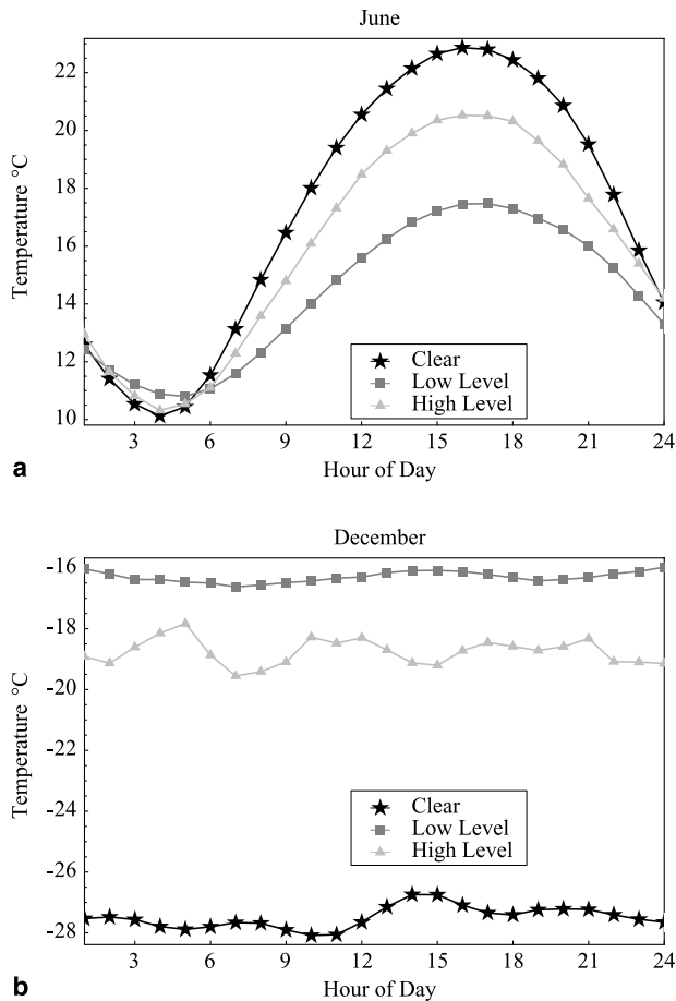
Fig. 10. Diurnal temperature variation for June (a) and December (b) for a clear day as well as days with high-level and low-level overcast, Fairbanks, Alaska
