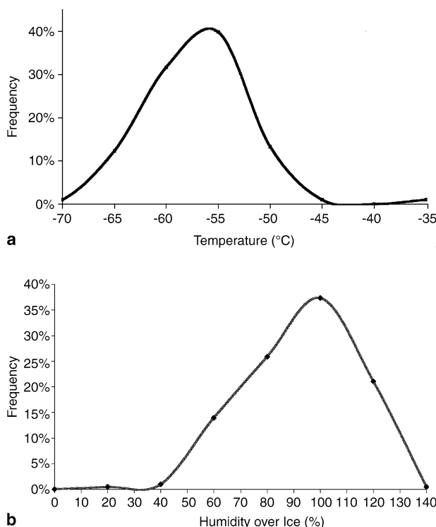
Fig. 5. Temperature (a) and relative humidity (b) at flight level for long lasting (>10 minutes) contrails at Fairbanks, Alaska
