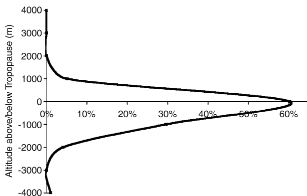
Fig. 4. Altitude distribution of longer lasting contrails (>10 minutes) in reference to the tropopause. Positive values refer to contrails in the stratosphere
