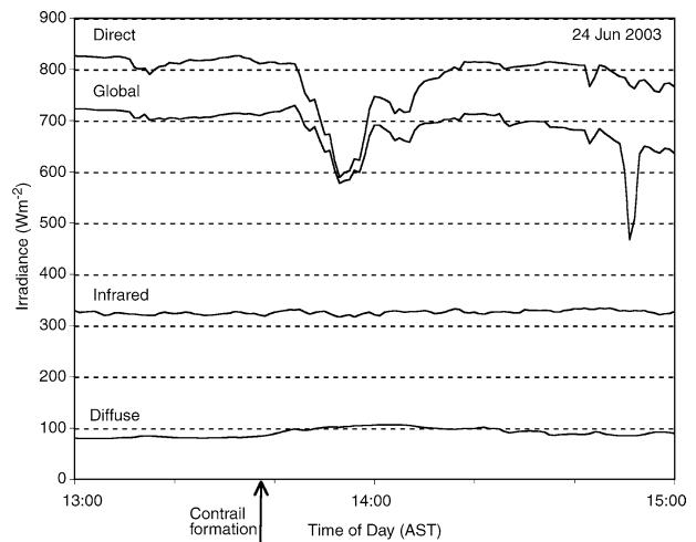
Fig. 7. The effect of a contrail on the radiation fluxes for a summer day (24 June 2003) at Fairbanks, Alaska
