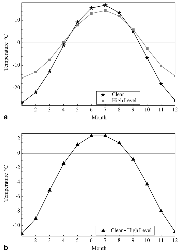
Fig. 9. Mean annual temperature course of Fairbanks for a clear day and a day with high-level cloudiness (a) and the temperature difference between the two (b) for Fairbanks, Alaska. Note, that with the exception of May through August, days with high-level cloudiness are warmer than clear days
