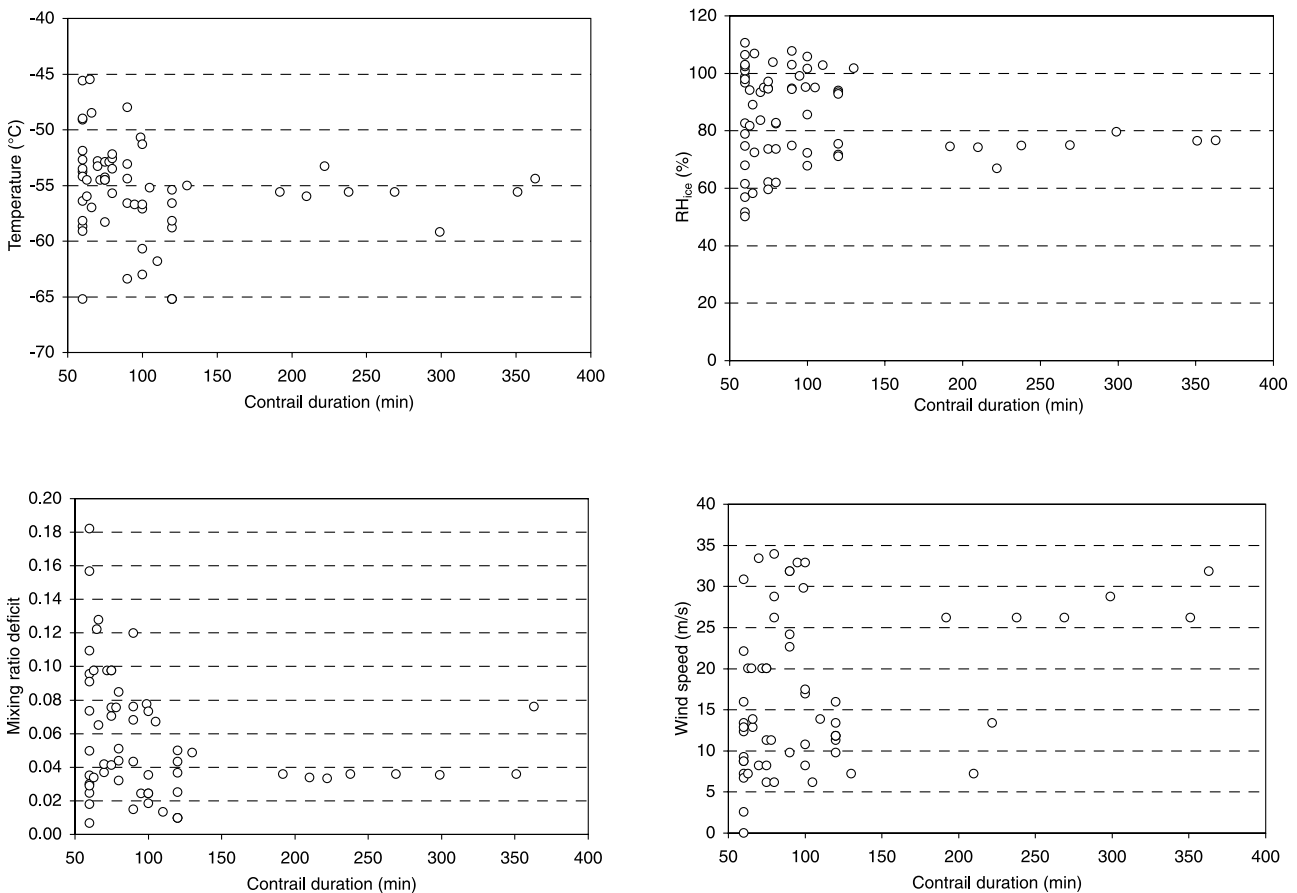
Fig. 6. Temperature, relative humidity, wind speed and saturation mixing ratio deficit as function of contrail duration for contrails lasting longer than 60 minutes, Fairbanks, Alaska
